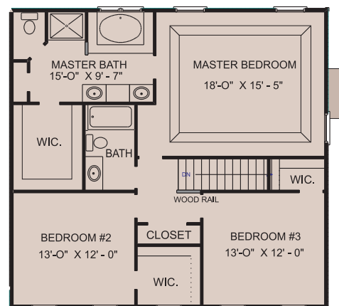
ELIZABETH AVERY 2ND FLOOR 34' - 0" X 32' - 0" 1088 SQ. FT.
