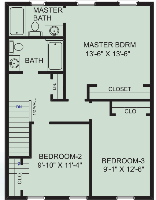
HERITAGE 24'-0" x 32' 768 SQ. FT.
