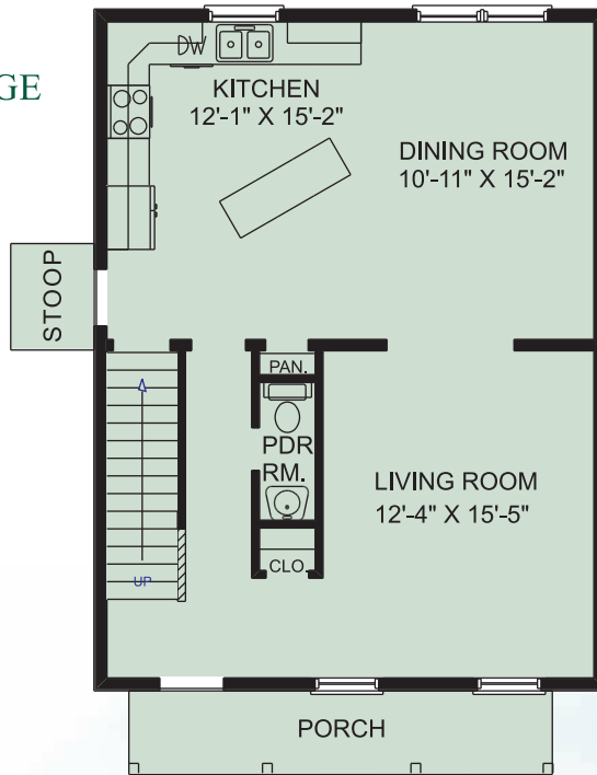
HERITAGE 24'-0" x 36'-0" 768 SQ. FT.
